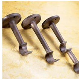
STANDARD, EXTENDED, DOUBLE BRACKET (left to right) Standard bracket projects 4.25" (for both diameters); Extended bracket projects 5.75" and 6.1" (for 1" and 1.5" rods respec- tively); Double bracket projects 4" and 7.5" (for both diameters)
