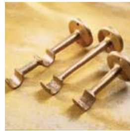
STANDARD, EXTENDED, DOUBLE BRACKET (right to left) Standard bracket projects 4" and 5"; Extended bracket projects 6.5" and 7.5"; Double bracket projects 7" and 8" (for 1" and 2" rods respectively)
