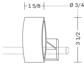
bracket
