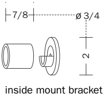
inside mount bracket
