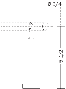
pass-through bracket extended
