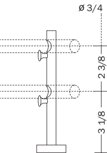
double rest-in bracket
