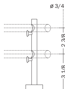
double rest-in bracket
