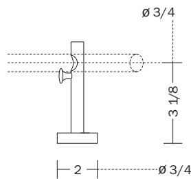
inside mount bracket
